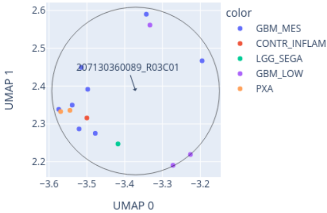
Close-up of UMAP for 207130360089_R03C01 reference: AllIDATv2_20210804_HPAP_Sarc.xlsx (19967 cases), 0 CpGs
