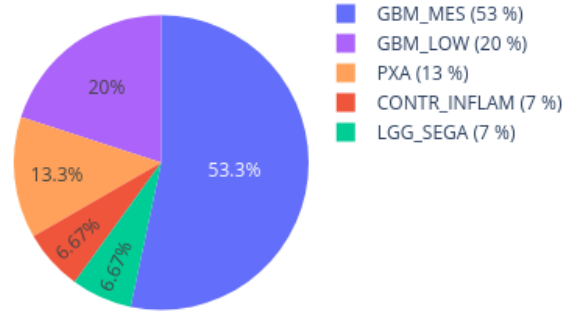
Neighbors in UMAP for 207130360089_R03C01 reference: AllIDATv2_20210804_HPAP_Sarc.xlsx (19967 cases), 0 CpGs
