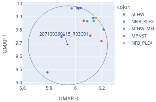
Close-up of UMAP for 207130360115_R03C01 reference: AllIDATv2_20210804_HPAP_Sarc.xlsx (19967 cases), 0 CpGs
