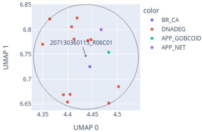
Close-up of UMAP for 207130360115_R06C01 reference: AllIDATv2_20210804_HPAP_Sarc.xlsx (19967 cases), 0 CpGs
