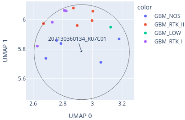
Close-up of UMAP for 207130360134_R07C01 reference: AllIDATv2_20210804_HPAP_Sarc.xlsx (19967 cases), 0 CpGs
