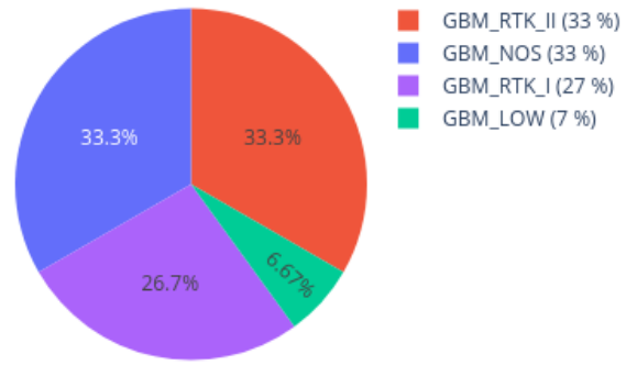
Neighbors in UMAP for 207130360134_R07C01 reference: AllIDATv2_20210804_HPAP_Sarc.xlsx (19967 cases), 0 CpGs
