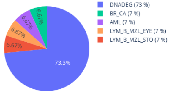
Neighbors in UMAP for 207130370025_R02C01 reference: AllIDATv2_20210804_HPAP_Sarc.xlsx (19967 cases), 0 CpGs
