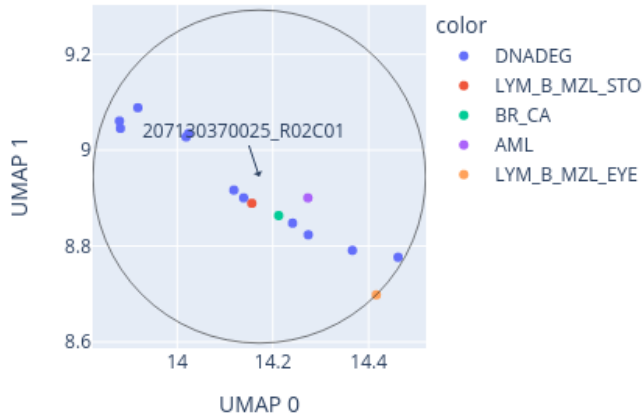
Close-up of UMAP for 207130370025_R02C01 reference: AllIDATv2_20210804_HPAP_Sarc.xlsx (19967 cases), 0 CpGs
