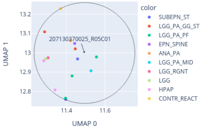
Close-up of UMAP for 207130370025_R05C01 reference: AllIDATv2_20210804_HPAP_Sarc.xlsx (19967 cases), 0 CpGs
