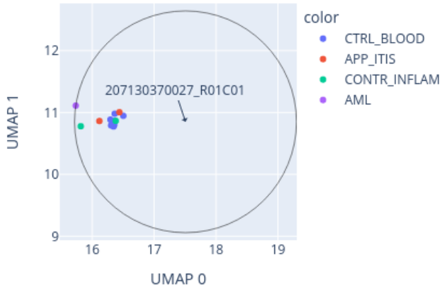
Close-up of UMAP for 207130370027_R01C01 reference: AllIDATv2_20210804_HPAP_Sarc.xlsx (19967 cases), 0 CpGs
