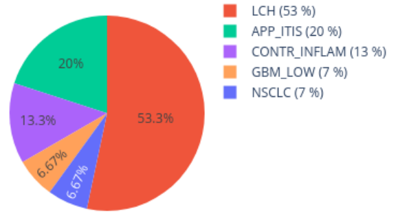
Neighbors in UMAP for 207130370034_R03C01 reference: AllIDATv2_20210804_HPAP_Sarc.xlsx (19967 cases), 0 CpGs
