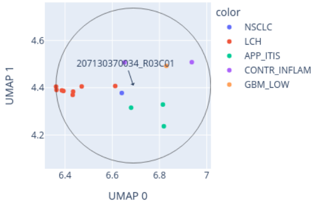
Close-up of UMAP for 207130370034_R03C01 reference: AllIDATv2_20210804_HPAP_Sarc.xlsx (19967 cases), 0 CpGs
