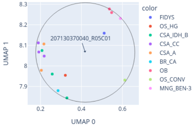
Close-up of UMAP for 207130370040_R05C01 reference: AllIDATv2_20210804_HPAP_Sarc.xlsx (19967 cases), 0 CpGs
