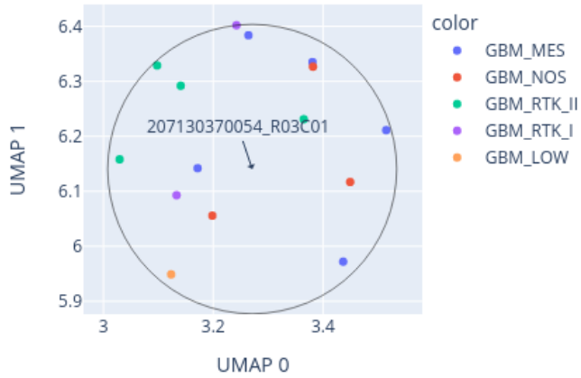
Close-up of UMAP for 207130370054_R03C01 reference: AllIDATv2_20210804_HPAP_Sarc.xlsx (19967 cases), 0 CpGs
