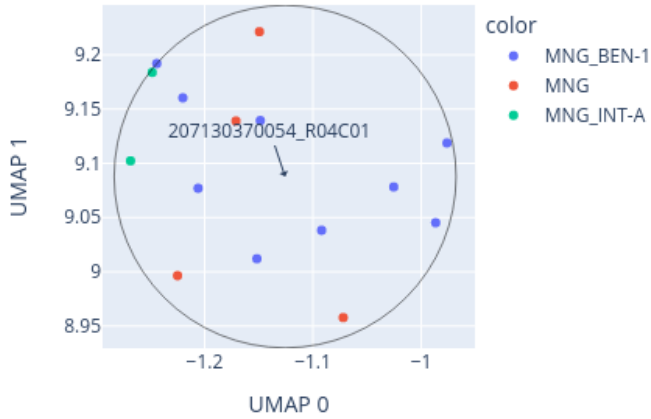
Close-up of UMAP for 207130370054_R04C01 reference: AllIDATv2_20210804_HPAP_Sarc.xlsx (19967 cases), 0 CpGs
