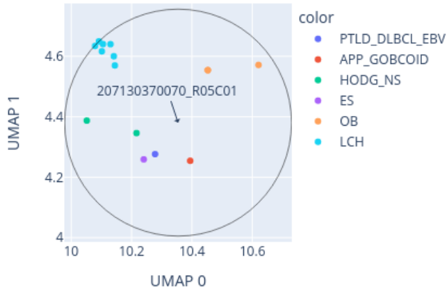
Close-up of UMAP for 207130370070_R05C01 reference: AllIDATv2_20210804_HPAP_Sarc.xlsx (19967 cases), 0 CpGs
