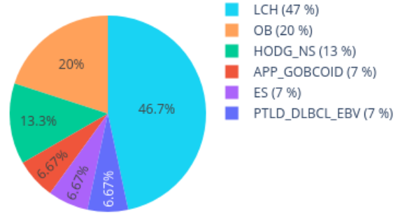
Neighbors in UMAP for 207130370070_R05C01 reference: AllIDATv2_20210804_HPAP_Sarc.xlsx (19967 cases), 0 CpGs
