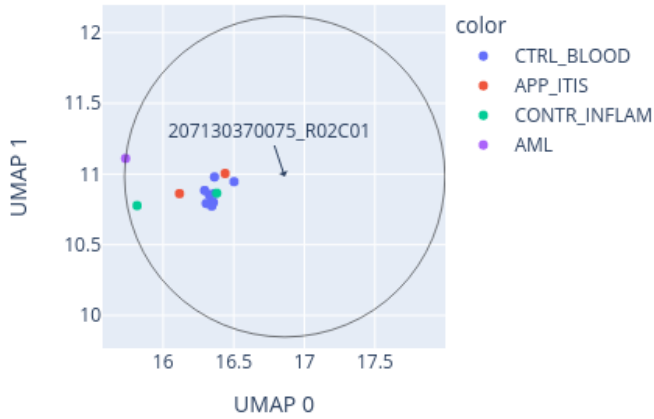
Close-up of UMAP for 207130370075_R02C01 reference: AllIDATv2_20210804_HPAP_Sarc.xlsx (19967 cases), 0 CpGs
