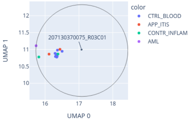
Close-up of UMAP for 207130370075_R03C01 reference: AllIDATv2_20210804_HPAP_Sarc.xlsx (19967 cases), 0 CpGs
