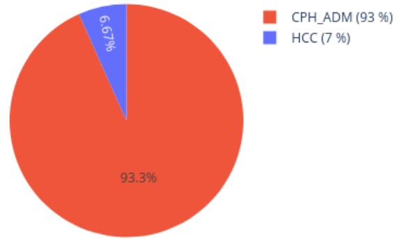
Neighbors in UMAP for 207130370076_R03C01 reference: AllIDATv2_20210804_HPAP_Sarc.xlsx (19967 cases), 0 CpGs
