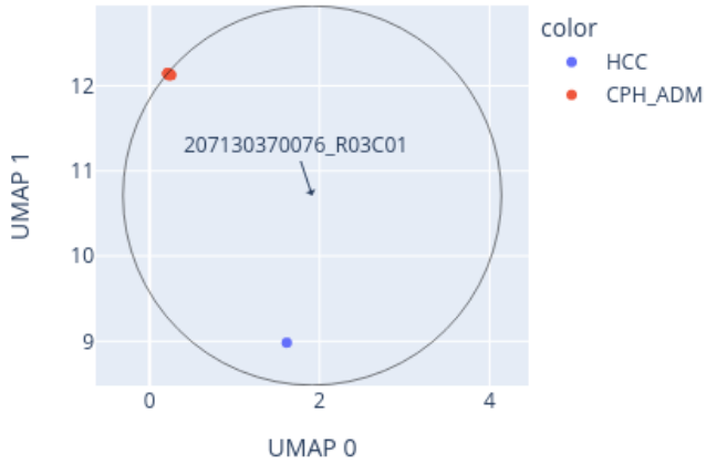
Close-up of UMAP for 207130370076_R03C01 reference: AllIDATv2_20210804_HPAP_Sarc.xlsx (19967 cases), 0 CpGs
