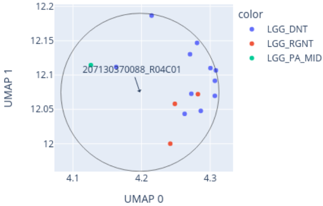
Close-up of UMAP for 207130370088_R04C01 reference: AllIDATv2_20210804_HPAP_Sarc.xlsx (19967 cases), 0 CpGs
