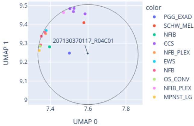
Close-up of UMAP for 207130370117_R04C01 reference: AllIDATv2_20210804_HPAP_Sarc.xlsx (19967 cases), 0 CpGs
