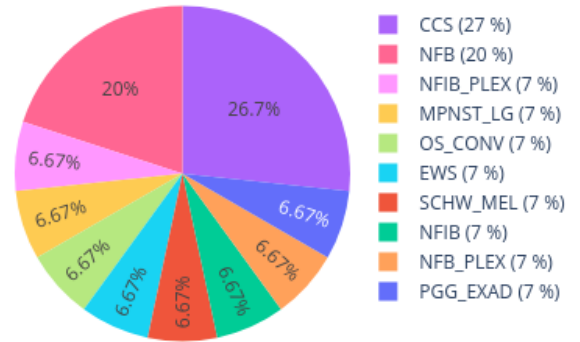
Neighbors in UMAP for 207130370117_R04C01 reference: AllIDATv2_20210804_HPAP_Sarc.xlsx (19967 cases), 0 CpGs
