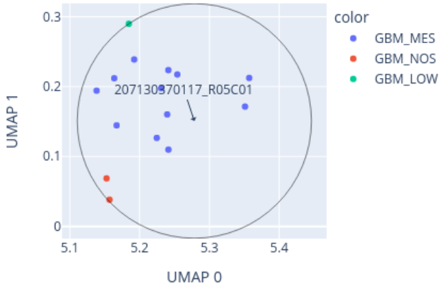
Close-up of UMAP for 207130370117_R05C01 reference: AllIDATv2_20210804_HPAP_Sarc.xlsx (19967 cases), 0 CpGs
