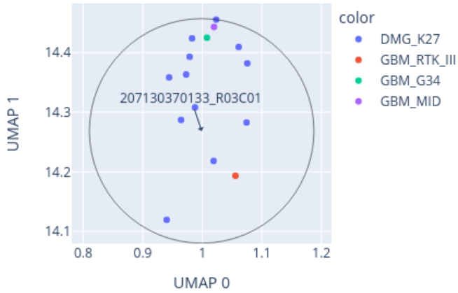
Close-up of UMAP for 207130370133_R03C01 reference: AllIDATv2_20210804_HPAP_Sarc.xlsx (19967 cases), 0 CpGs
