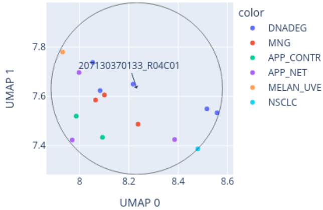
Close-up of UMAP for 207130370133_R04C01 reference: AllIDATv2_20210804_HPAP_Sarc.xlsx (19967 cases), 0 CpGs
