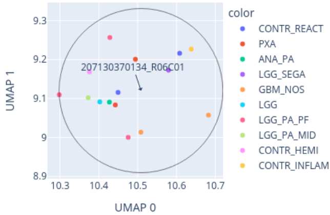
Close-up of UMAP for 207130370134_R06C01 reference: AllIDATv2_20210804_HPAP_Sarc.xlsx (19967 cases), 0 CpGs
