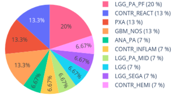
Neighbors in UMAP for 207130370134_R06C01 reference: AllIDATv2_20210804_HPAP_Sarc.xlsx (19967 cases), 0 CpGs
