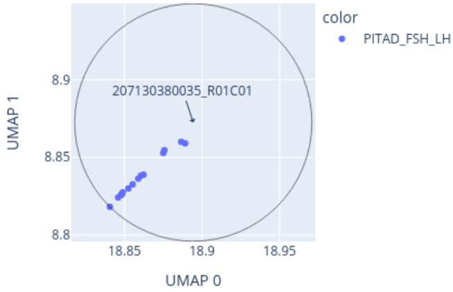
Close-up of UMAP for 207130380035_R01C01 reference: AllIDATv2_20210804_HPAP_Sarc.xlsx (19967 cases), 0 CpGs
