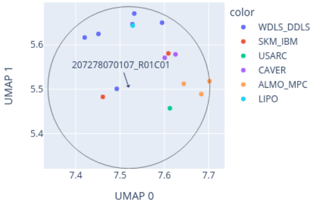
Close-up of UMAP for 207278070107_R01C01 reference: AllIDATv2_20210804_HPAP_Sarc.xlsx (19967 cases), 0 CpGs
