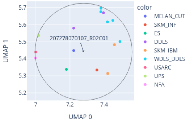
Close-up of UMAP for 207278070107_R02C01 reference: AllIDATv2_20210804_HPAP_Sarc.xlsx (19967 cases), 0 CpGs
