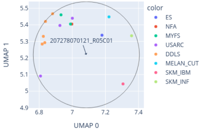
Close-up of UMAP for 207278070121_R05C01 reference: AllIDATv2_20210804_HPAP_Sarc.xlsx (19967 cases), 0 CpGs
