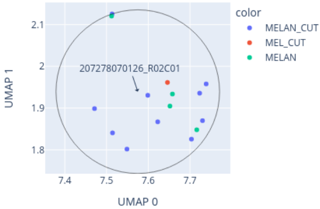
Close-up of UMAP for 207278070126_R02C01 reference: AllIDATv2_20210804_HPAP_Sarc.xlsx (19967 cases), 0 CpGs
