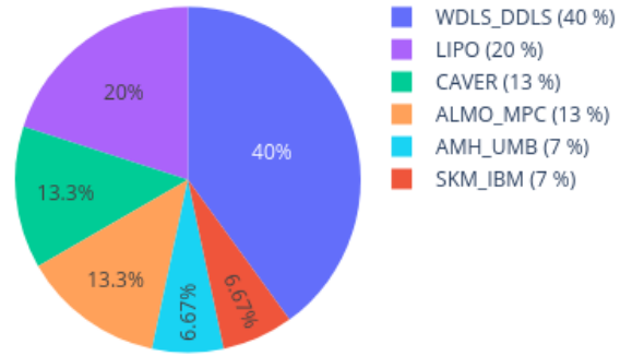
Neighbors in UMAP for 207310410093_R06C01 reference: AllIDATv2_20210804_HPAP_Sarc.xlsx (19967 cases), 0 CpGs
