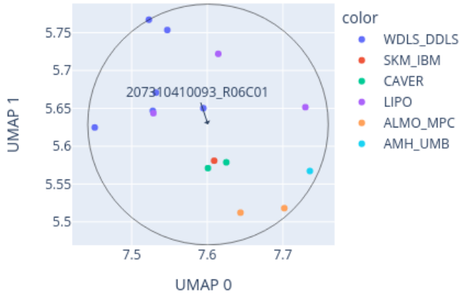
Close-up of UMAP for 207310410093_R06C01 reference: AllIDATv2_20210804_HPAP_Sarc.xlsx (19967 cases), 0 CpGs
