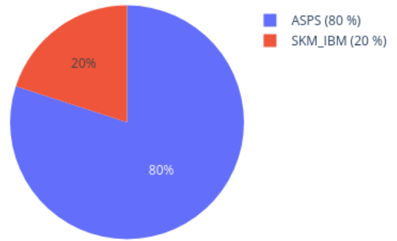
Neighbors in UMAP for 207310410114_R04C01 reference: AllIDATv2_20210804_HPAP_Sarc.xlsx (19967 cases), 0 CpGs
