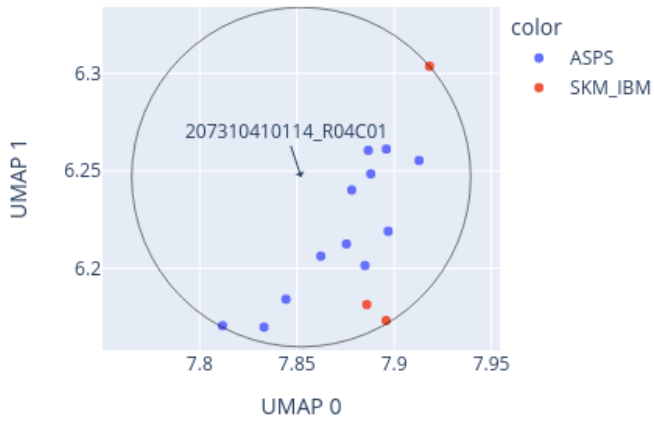
Close-up of UMAP for 207310410114_R04C01 reference: AllIDATv2_20210804_HPAP_Sarc.xlsx (19967 cases), 0 CpGs
