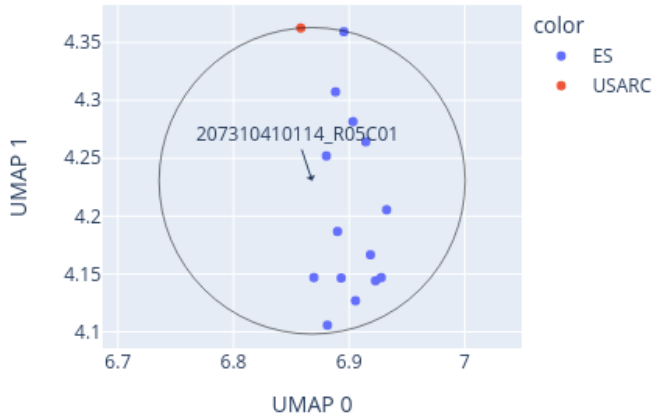
Close-up of UMAP for 207310410114_R05C01 reference: AllIDATv2_20210804_HPAP_Sarc.xlsx (19967 cases), 0 CpGs
