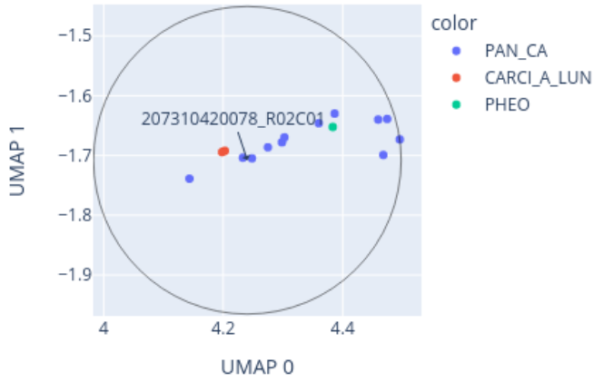
Close-up of UMAP for 207310420078_R02C01 reference: AllIDATv2_20210804_HPAP_Sarc.xlsx (19967 cases), 0 CpGs
