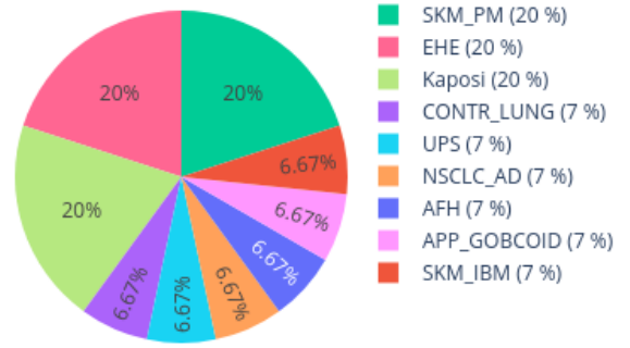
Neighbors in UMAP for 207310420078_R05C01 reference: AllIDATv2_20210804_HPAP_Sarc.xlsx (19967 cases), 0 CpGs
