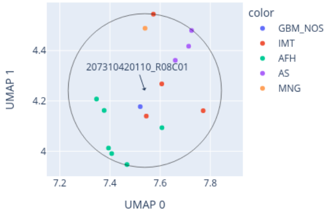
Close-up of UMAP for 207310420110_R08C01 reference: AllIDATv2_20210804_HPAP_Sarc.xlsx (19967 cases), 0 CpGs
