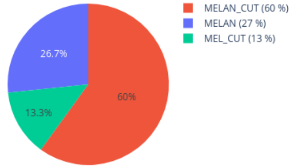
Neighbors in UMAP for 207357020134_R02C01 reference: AllIDATv2_20210804_HPAP_Sarc.xlsx (19967 cases), 0 CpGs
