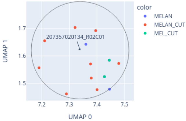
Close-up of UMAP for 207357020134_R02C01 reference: AllIDATv2_20210804_HPAP_Sarc.xlsx (19967 cases), 0 CpGs
