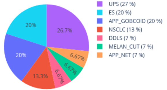
Neighbors in UMAP for 207361110158_R04C01 reference: AllIDATv2_20210804_HPAP_Sarc.xlsx (19967 cases), 0 CpGs
