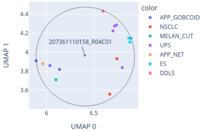
Close-up of UMAP for 207361110158_R04C01 reference: AllIDATv2_20210804_HPAP_Sarc.xlsx (19967 cases), 0 CpGs
