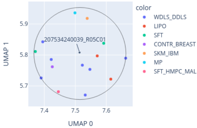
Close-up of UMAP for 207534240039_R05C01 reference: AllIDATv2_20210804_HPAP_Sarc.xlsx (19967 cases), 0 CpGs
