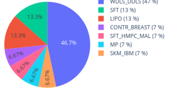
Neighbors in UMAP for 207534240039_R05C01 reference: AllIDATv2_20210804_HPAP_Sarc.xlsx (19967 cases), 0 CpGs
