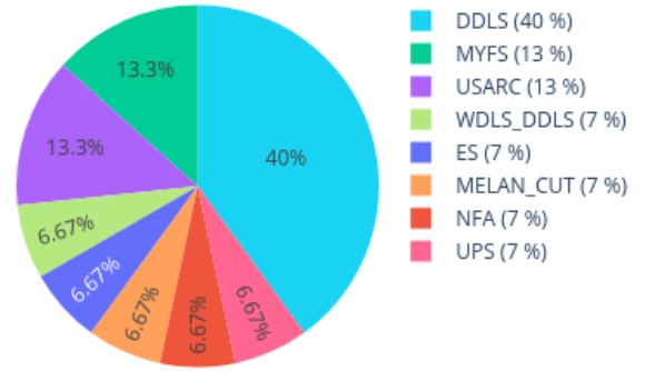
Neighbors in UMAP for 207534240089_R01C01 reference: AllIDATv2_20210804_HPAP_Sarc.xlsx (19967 cases), 0 CpGs
