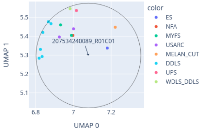
Close-up of UMAP for 207534240089_R01C01 reference: AllIDATv2_20210804_HPAP_Sarc.xlsx (19967 cases), 0 CpGs
