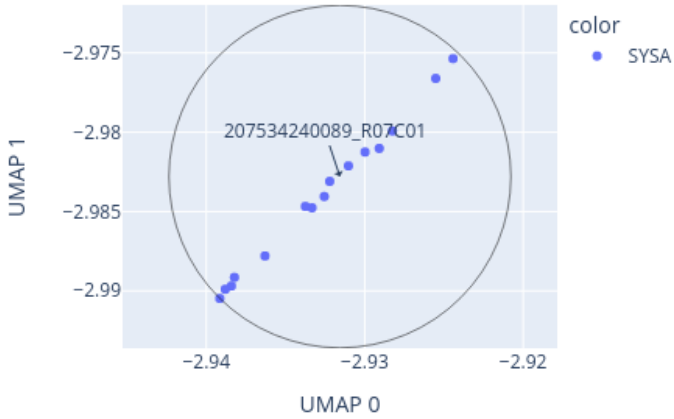
Close-up of UMAP for 207534240089_R07C01 reference: AllIDATv2_20210804_HPAP_Sarc.xlsx (19967 cases), 0 CpGs
