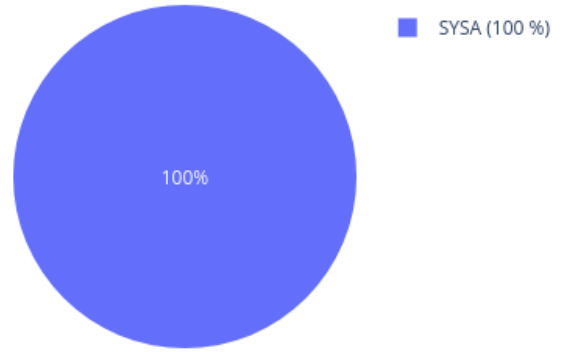
Neighbors in UMAP for 207534240089_R07C01 reference: AllIDATv2_20210804_HPAP_Sarc.xlsx (19967 cases), 0 CpGs
