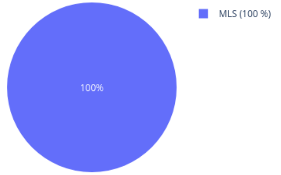
Neighbors in UMAP for 207744350056_R04C01 reference: AllIDATv2_20210804_HPAP_Sarc.xlsx (19967 cases), 0 CpGs
