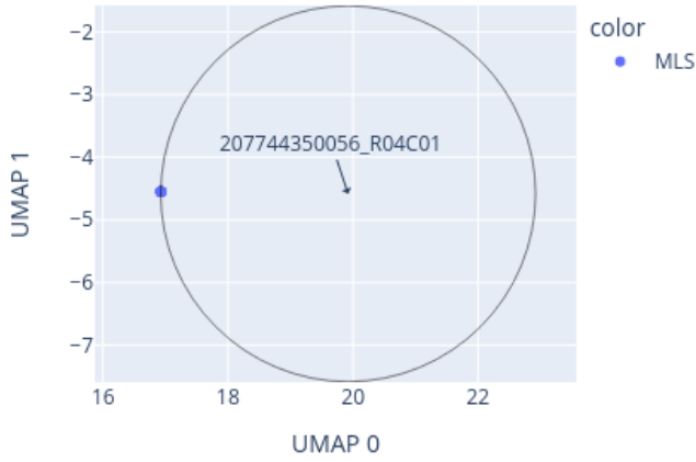
Close-up of UMAP for 207744350056_R04C01 reference: AllIDATv2_20210804_HPAP_Sarc.xlsx (19967 cases), 0 CpGs
