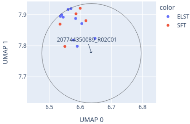
Close-up of UMAP for 207744350089_R02C01 reference: AllIDATv2_20210804_HPAP_Sarc.xlsx (19967 cases), 0 CpGs
