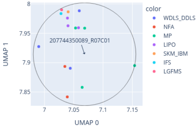
Close-up of UMAP for 207744350089_R07C01 reference: AllIDATv2_20210804_HPAP_Sarc.xlsx (19967 cases), 0 CpGs
