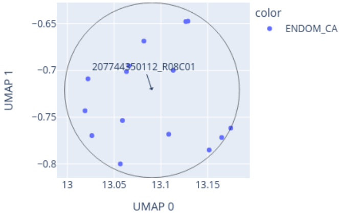
Close-up of UMAP for 207744350112_R08C01 reference: AllIDATv2_20210804_HPAP_Sarc.xlsx (19967 cases), 0 CpGs
