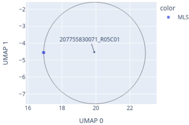
Close-up of UMAP for 207755830071_R05C01 reference: AllIDATv2_20210804_HPAP_Sarc.xlsx (19967 cases), 0 CpGs
