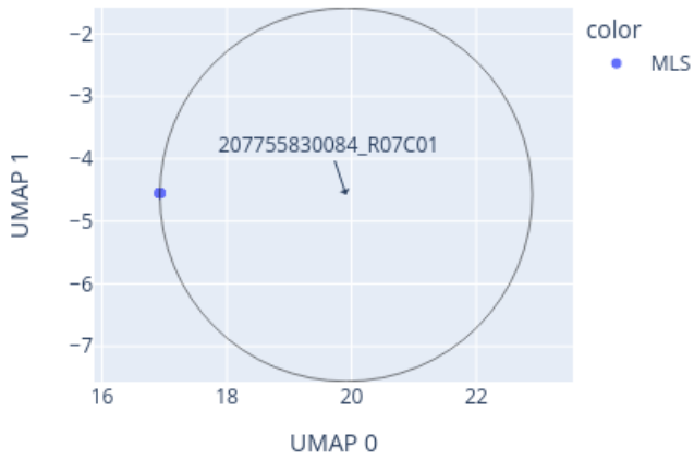
Close-up of UMAP for 207755830084_R07C01 reference: AllIDATv2_20210804_HPAP_Sarc.xlsx (19967 cases), 0 CpGs
