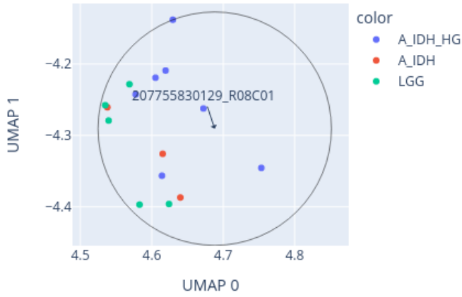
Close-up of UMAP for 207755830129_R08C01 reference: AllIDATv2_20210804_HPAP_Sarc.xlsx (19967 cases), 0 CpGs
