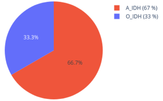
Neighbors in UMAP for 207755830135_R05C01 reference: AllIDATv2_20210804_HPAP_Sarc.xlsx (19967 cases), 0 CpGs
