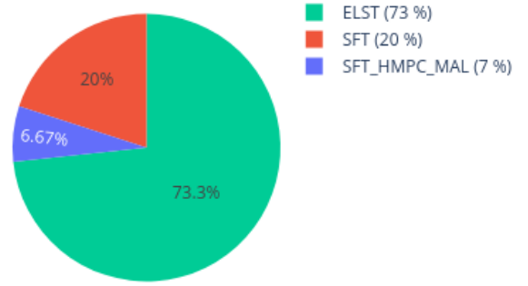
Neighbors in UMAP for 207758440072_R07C01 reference: AllIDATv2_20210804_HPAP_Sarc.xlsx (19967 cases), 0 CpGs
