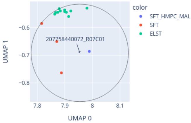
Close-up of UMAP for 207758440072_R07C01 reference: AllIDATv2_20210804_HPAP_Sarc.xlsx (19967 cases), 0 CpGs
