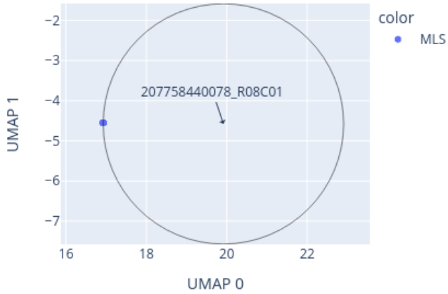
Close-up of UMAP for 207758440078_R08C01 reference: AllIDATv2_20210804_HPAP_Sarc.xlsx (19967 cases), 0 CpGs
