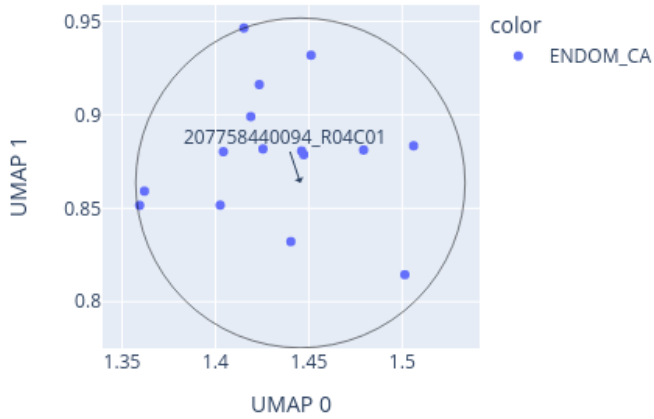
Close-up of UMAP for 207758440094_R04C01 reference: AllIDATv2_20210804_HPAP_Sarc.xlsx (19967 cases), 0 CpGs
