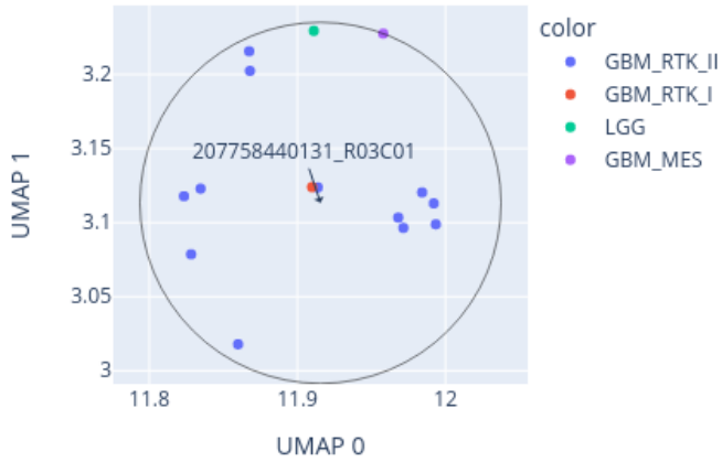
Close-up of UMAP for 207758440131_R03C01 reference: AllIDATv2_20210804_HPAP_Sarc.xlsx (19967 cases), 0 CpGs
