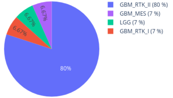
Neighbors in UMAP for 207758440131_R03C01 reference: AllIDATv2_20210804_HPAP_Sarc.xlsx (19967 cases), 0 CpGs
