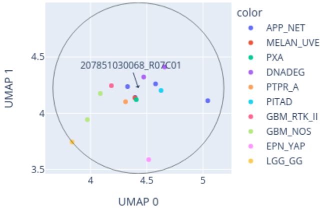
Close-up of UMAP for 207851030068_R07C01 reference: AllIDATv2_20210804_HPAP_Sarc.xlsx (19967 cases), 0 CpGs
